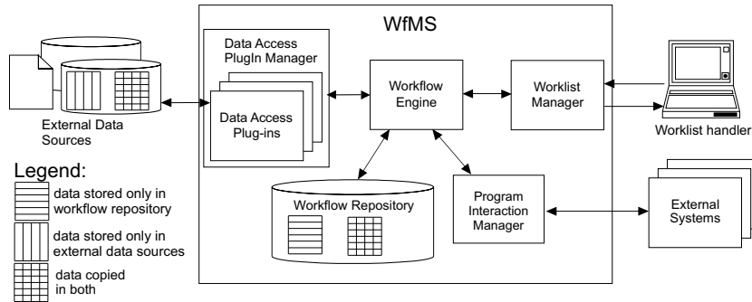
Fig. 1. WfMS architecture
